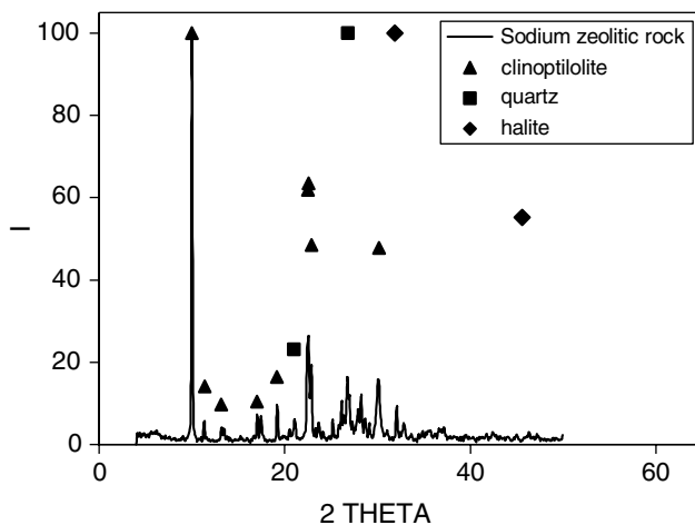
Figure 2. Powder diffraction pattern of the zeolitic rock treated with sodium chloride solution.
