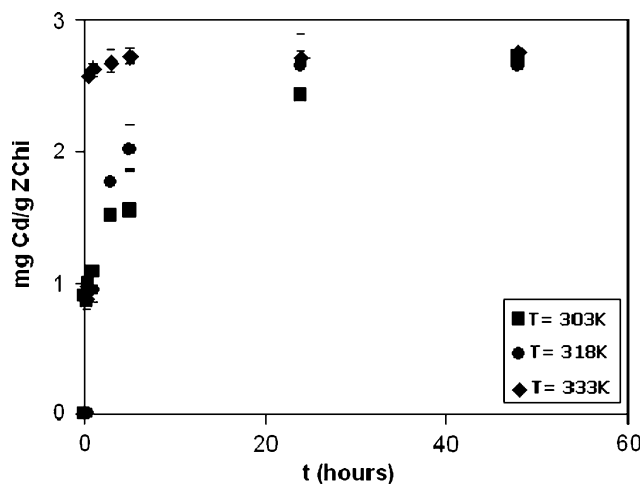
Figure 4. Sorption behavior of \text{Cd}^{2+} vs. time (h) at different temperatures.
